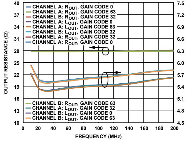
Figure 34. Differential Series Output Resistance and Inductance vs. Frequency
